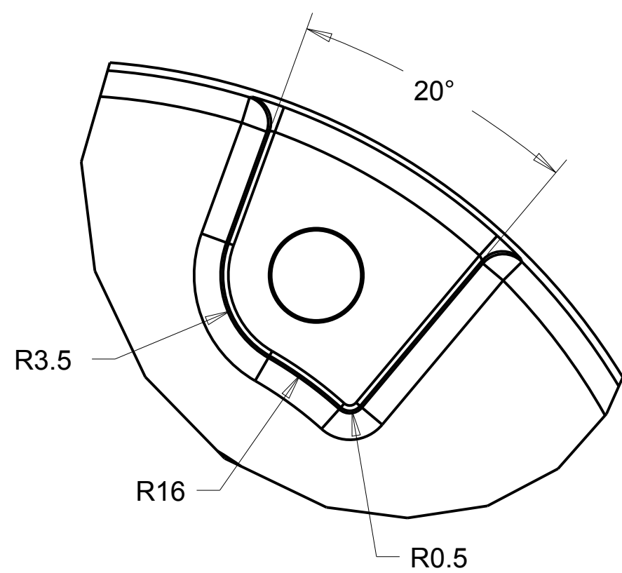
DETAIL A SCALE 5.000
